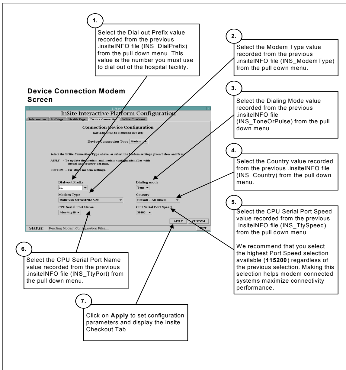
Figure 5 Insite Interactive Platform Configuration Utility Device Connection Tab – Modem Setup
